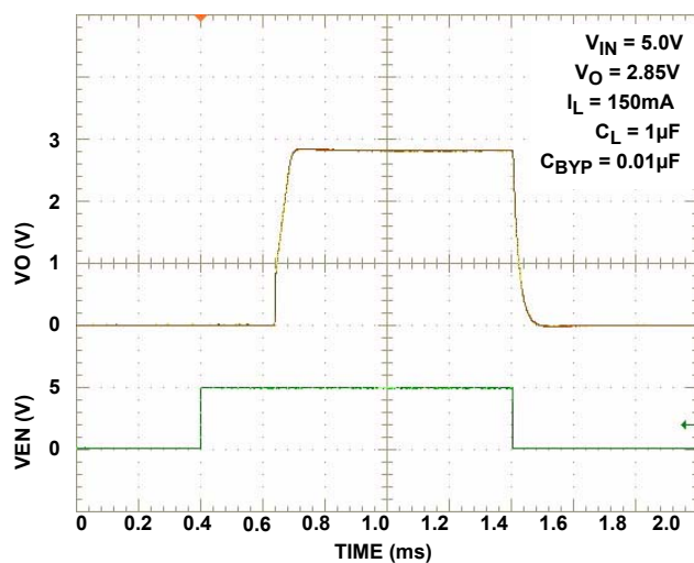
FIGURE 13. TURN-ON/TURN-OFF RESPONSE
