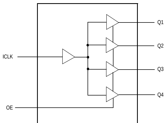
Figure 1. Logic Diagram
