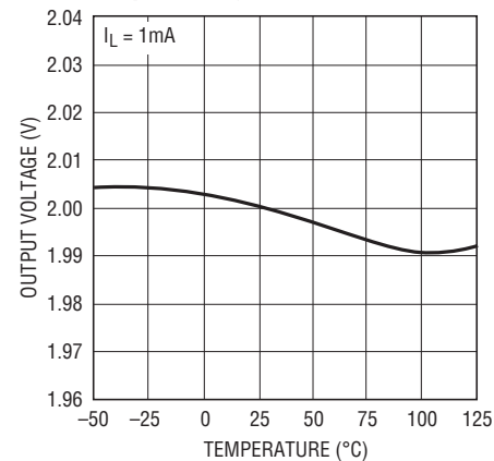
LT1761-2 Output Voltage
