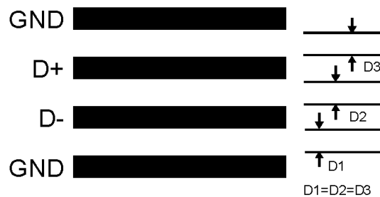
Figure 17. Ideal Diode Trace Layout
