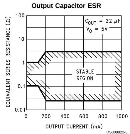
FIGURE 1. ESR Limits
