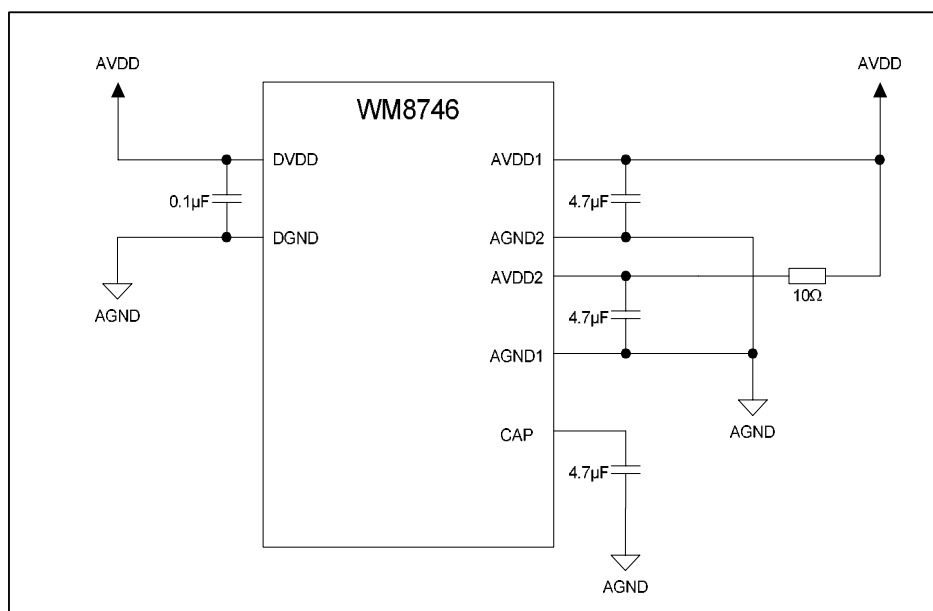
Figure 26 Decoupling Example 2
