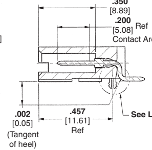
Section K-K
