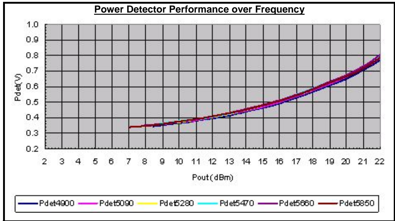
Figure 3: SE5012T Power Detector Characteristic
