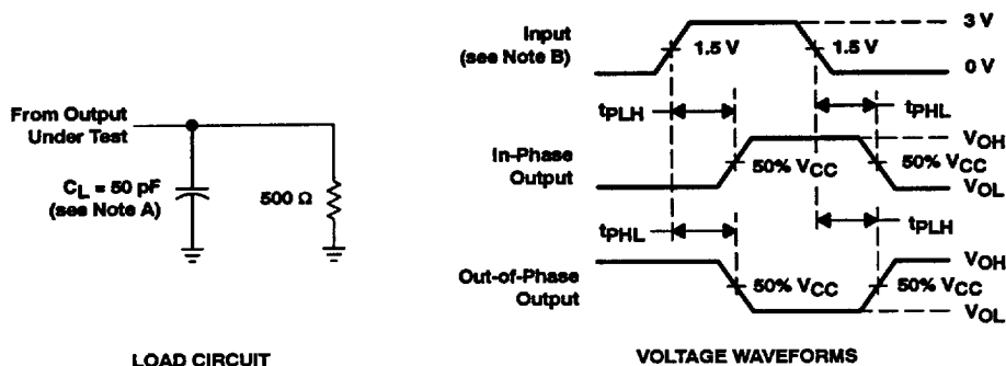
Figure 1. Load Circuit and Voltage Waveforms
