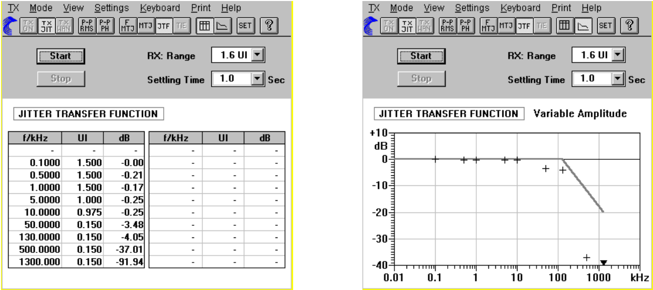
Figure A4: STM-1e jitter transfer test result
