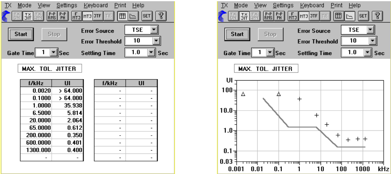
Figure A3: STM-1e jitter tolerance test result
