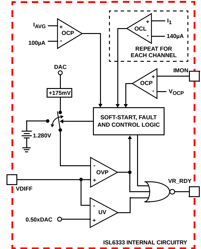
FIGURE 18. POWER GOOD AND PROTECTION CIRCUITRY
