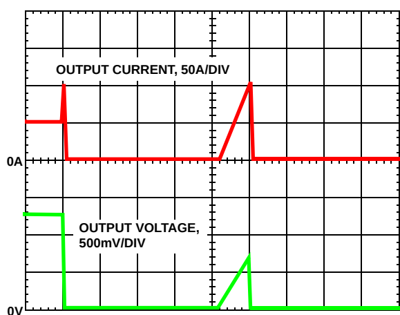
FIGURE 19. OVERCURRENT BEHAVIOR IN HICCUP MODE
