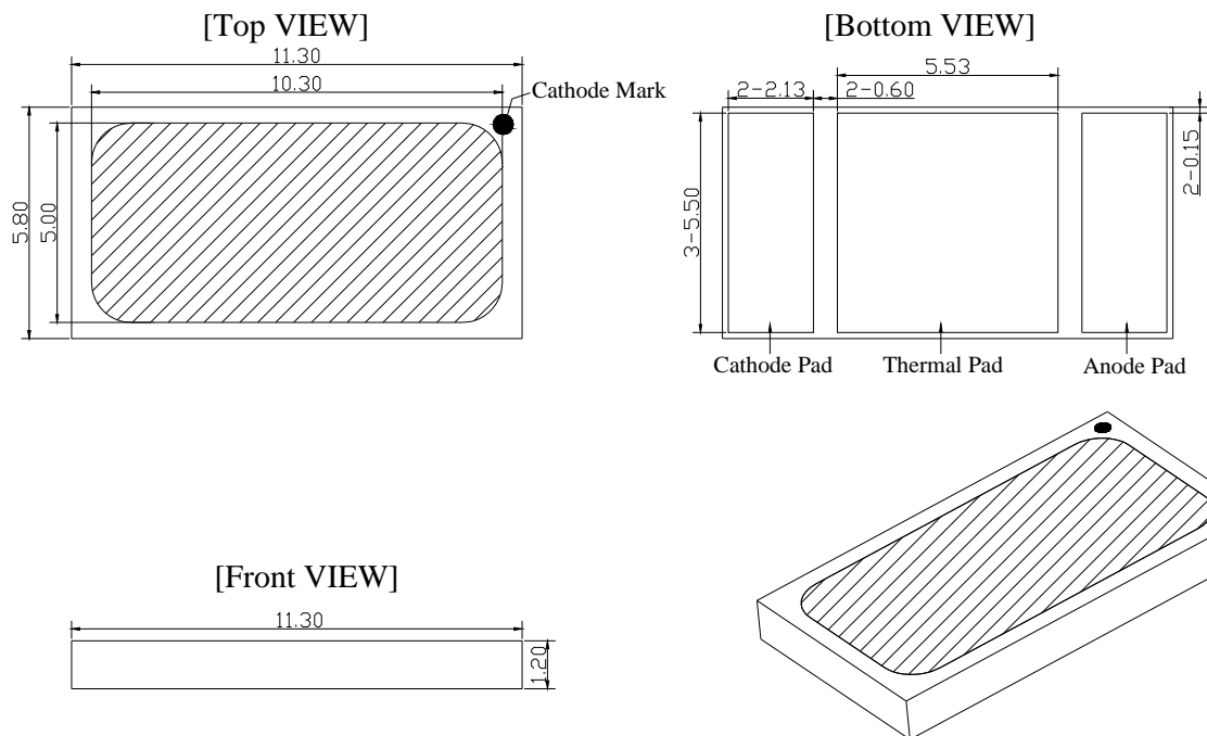
[Package Outlines]
