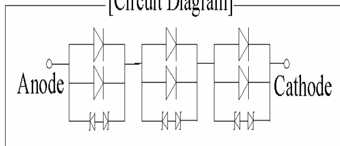
[Circuit Diagram]
