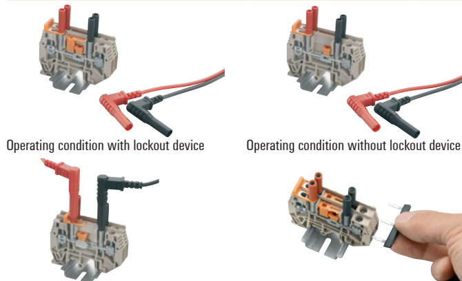
Testing condition with open disconnecting slider
