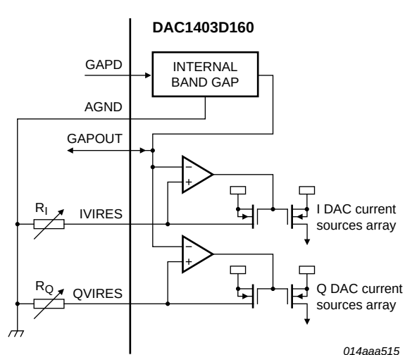
Fig 4. Internal reference configuration
