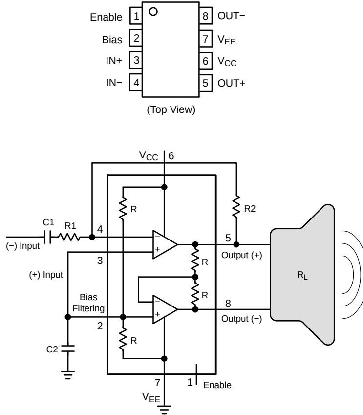
Figure 1. Block Diagram
