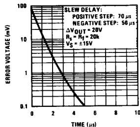
Inverter Final Settling Time
