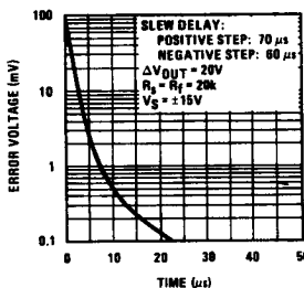
Follower Final Settling Time
