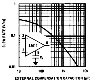
Slew Rate
