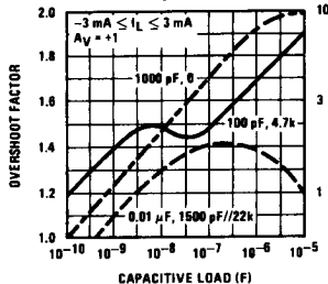
Stability With Over-Compensation
