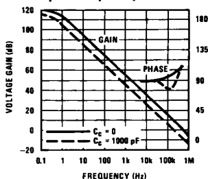
Open Loop Response
