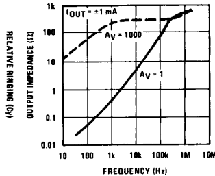
Closed Loop Output Impedance
