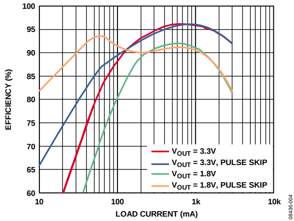
Figure 4. Efficiency vs. Load, V_{IN} = 5V and f_{SW} = 300\text{ kHz} ; V_{OUT} = 3.3V , Inductor Cooper Bussmann DR1050-8R2-R, 8.2\mu\text{H} , 15\text{ m}\Omega ; V_{OUT} = 1.8V , Inductor TOKO FDV0620-4R7M, 4.7\mu\text{H} , 53\text{ m}\Omega
