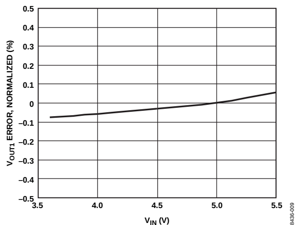
Figure 9. Line Regulation, Channel 1: Load Current = 3 A and f_{SW} = 600 kHz
