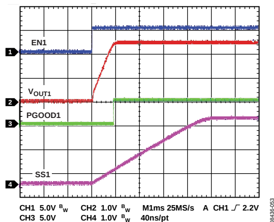
Figure 53. Power-Good Signal
