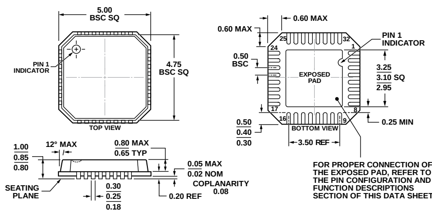
Figure 77. 32-Lead Lead Frame Chip Scale Package [LFCSP_VQ] 5 mm × 5 mm Body, Very Thin Quad (CP-32-2) Dimensions shown in millimeters
