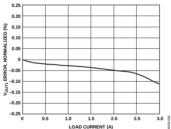
Figure 8. Load Regulation, Channel 1: V_{IN} = 5 V, f_{SW} = 600 kHz, and T_A = 25^\circ\text{C}
