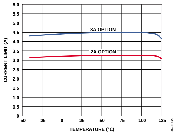
Figure 29. Peak Current Limit vs. Temperature, V_{IN} = 5\text{ V}
