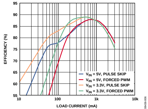
Figure 6. Efficiency vs. Load, V_{OUT} = 1.2V and f_{SW} = 1.2\text{ MHz} ; Inductor TOKO FDV0620-1R0M, 1.0\mu\text{H} , 14\text{ m}\Omega
