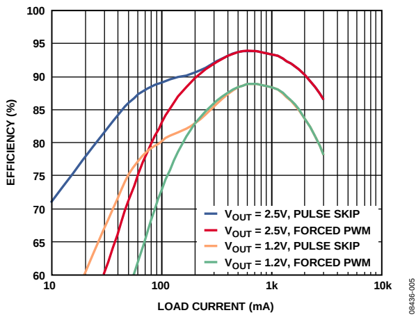
Figure 5. Efficiency vs. Load, V_{IN} = 5V and f_{SW} = 600\text{ kHz} ; V_{OUT} = 2.5V , Inductor TOKO FDV0620-3R3M, 3.3\mu\text{H} , 40\text{ m}\Omega ; V_{OUT} = 1.2V , Inductor TOKO FDV0620-2R2M, 2.2\mu\text{H} , 30\text{ m}\Omega
