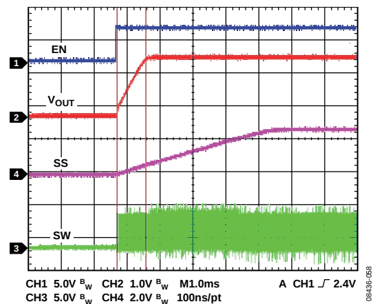
Figure 58. Soft Start
