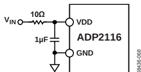
Figure 68. Low-Pass Filter at VDD
