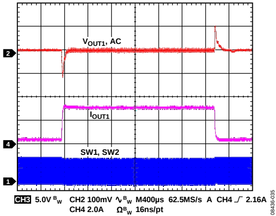
Figure 35. Load Transient Response in Pulse Skip Mode, Channel 1: 0.3 A to 3 A Load Step, V_{IN} = 5\text{ V} , V_{OUT} = 2.5\text{ V} , f_{SW} = 600\text{ kHz} (See Table 12 for the Circuit Details)
