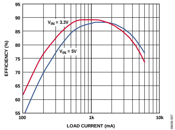
Figure 7. Efficiency, Combined Dual-Phase Output, V_{OUT} = 1.2V and f_{SW} = 1.2\text{ MHz} ; Inductor TOKO FDV0620-1R0M, 1.0\mu\text{H} , 14\text{ m}\Omega
