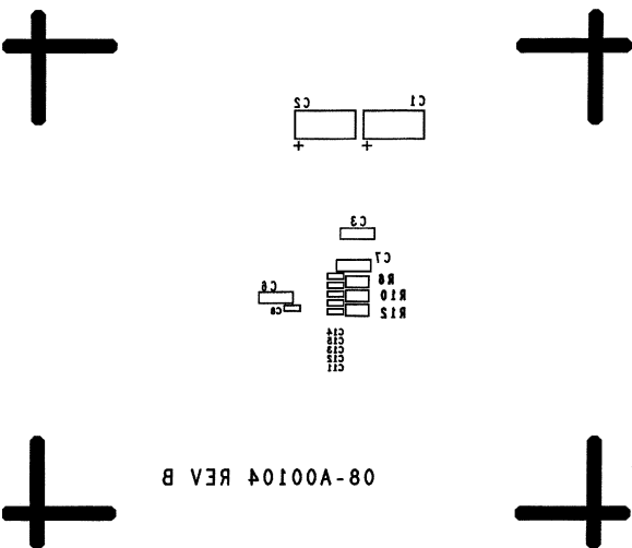
Figure 9. Silkscreen Bottom
