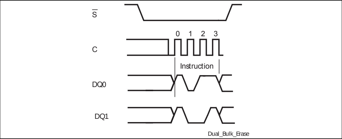
Figure 53. Bulk Erase instruction sequence DIO-SPI
