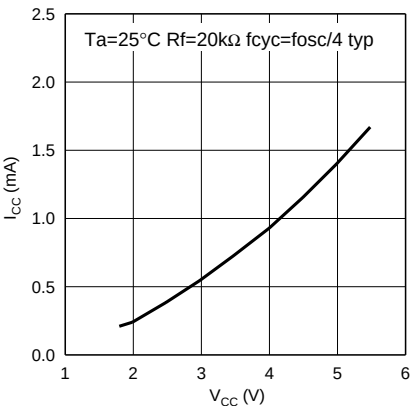
(b) I_{CC} vs. V_{CC} characteristic (resistance oscillation)
