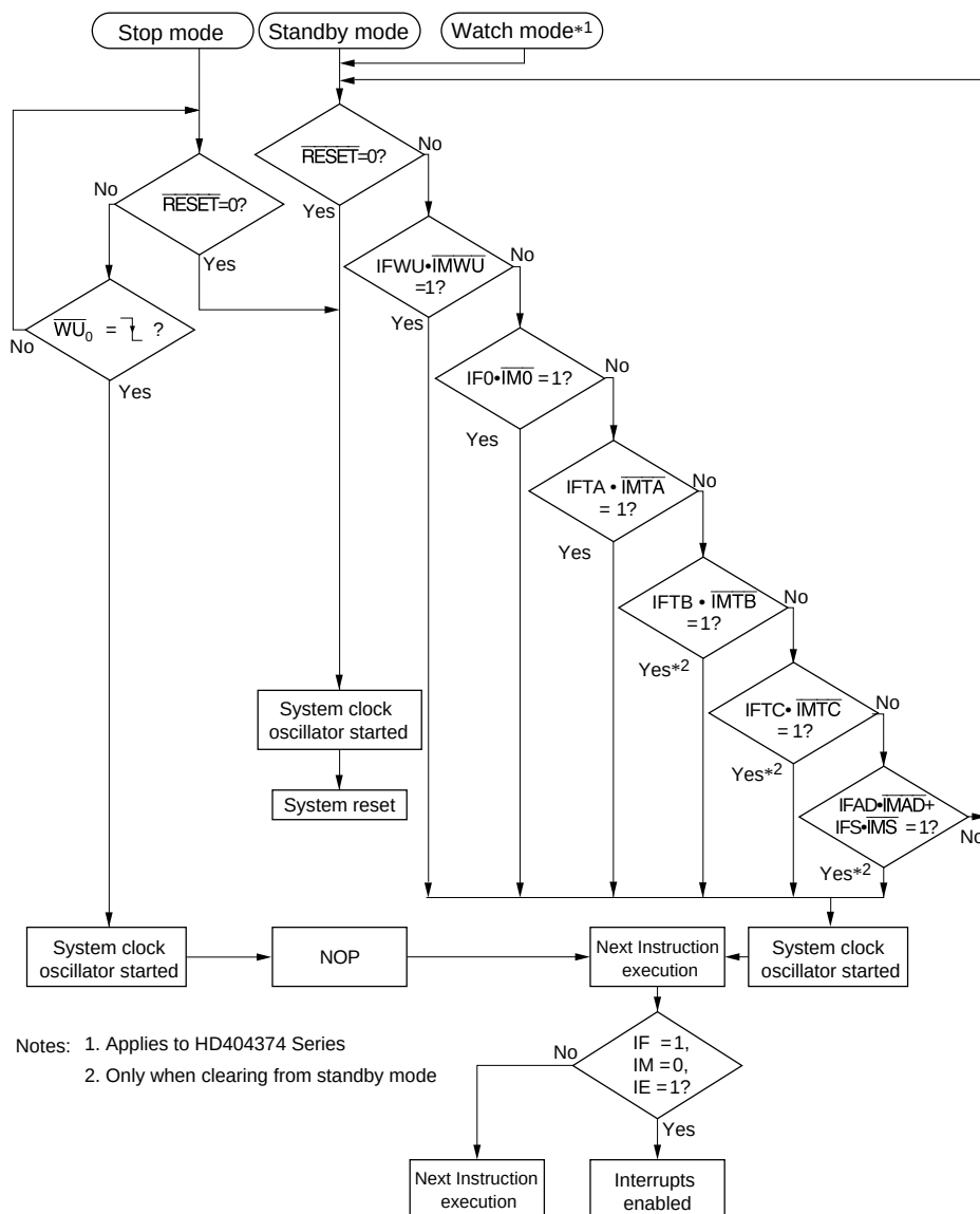
Figure 12 MCU Operation Flowchart
