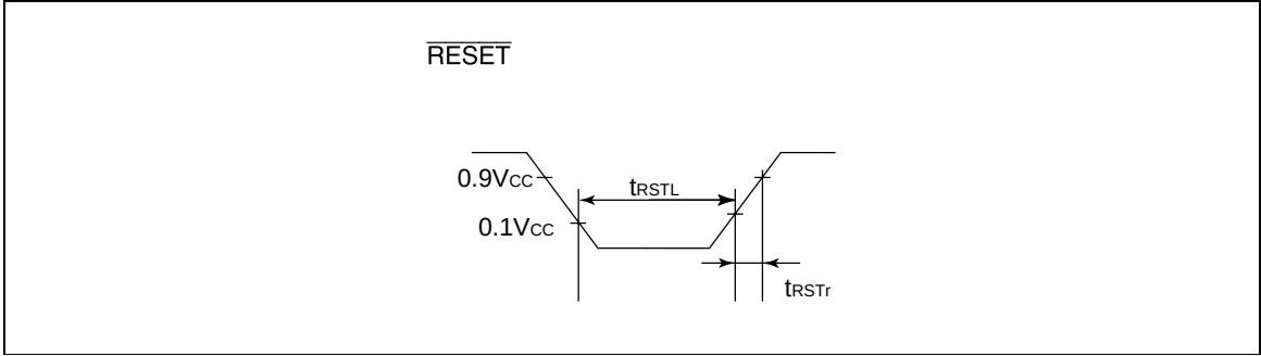
Figure 81 Reset Timing
