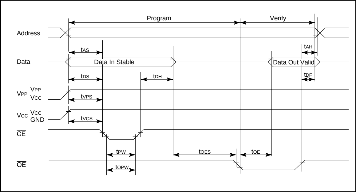
Figure 72 PROM Write/Verify Timing
