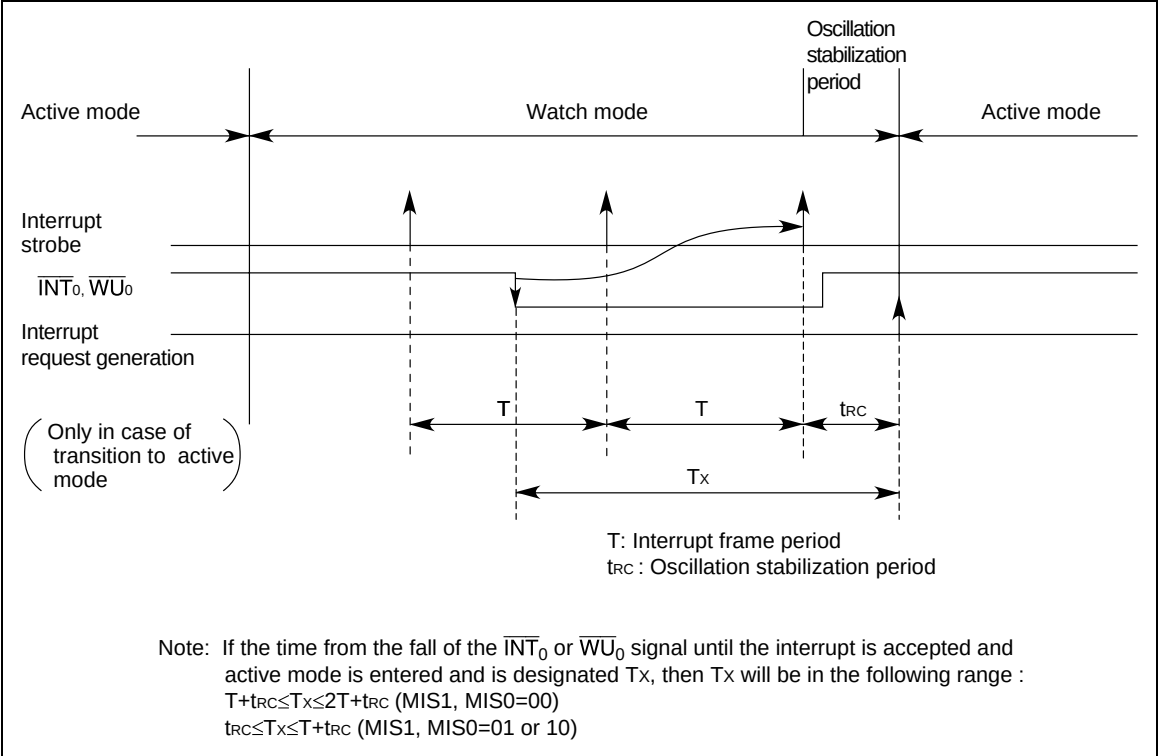
Figure 14 Interrupt Frame
