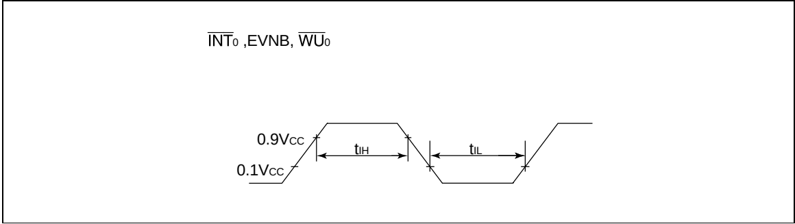
Figure 80 Interrupt Timing
