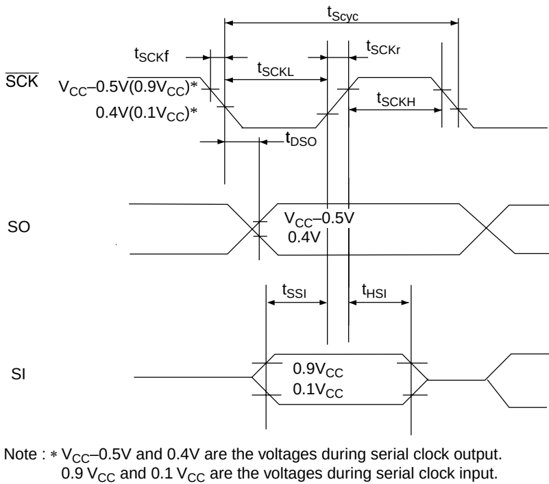
Figure 82 Serial Interface Timing
