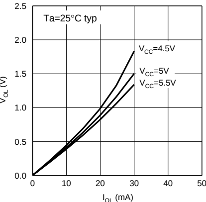
(e) V_{OL} vs. I_{OL} characteristic (pins D4 to D7)
