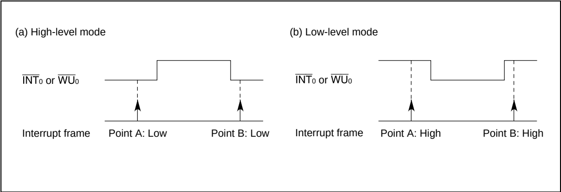
Figure 19 Sampling Examples
