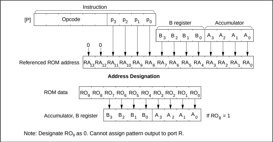
Figure 77 P Instruction
