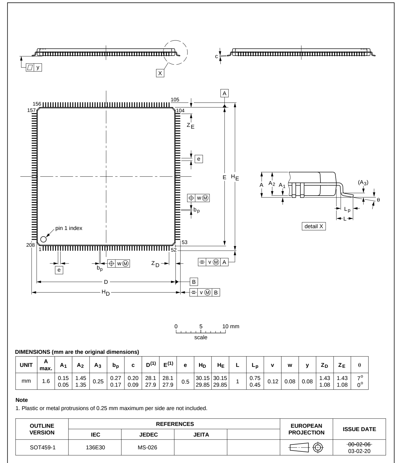
Fig 49. Package outline of the LQFP208 package
