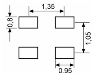
suggested soldering pad
