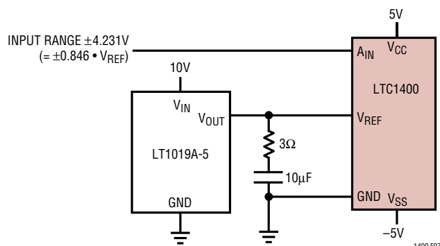
Figure 7. Supplying a 5V Reference Voltage to the LTC1400 with the LT1019A-5
