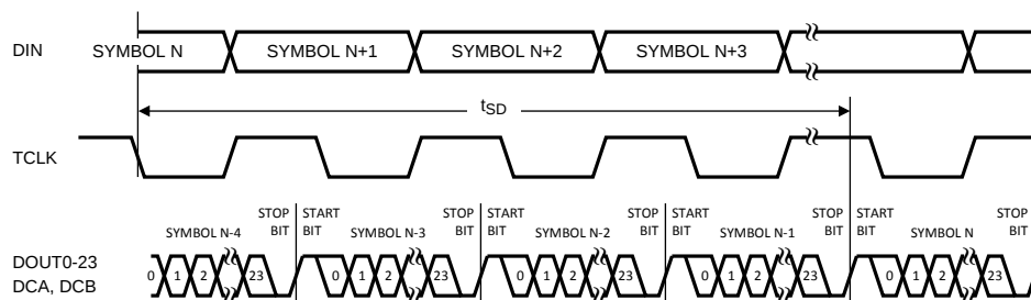
Figure 10. Serializer Delay
