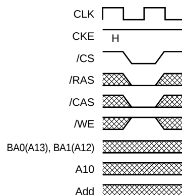
Fig.6 CBR (auto) refresh command
