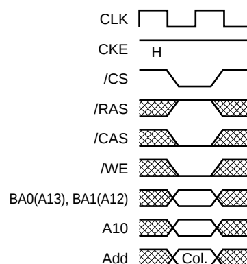
Fig.5 Column address and read command
