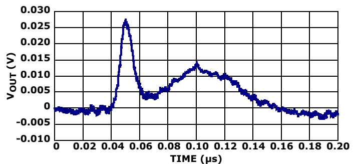
FIGURE 13. DYNAMIC RESPONSE, 15A TO 7A LOAD STEP
