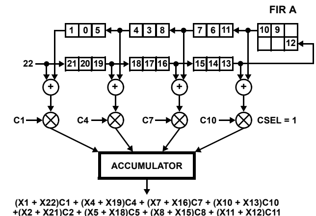
FIGURE 26B. COMPUTATIONAL FLOW AS DATA SAMPLE 22 IS CLOCKED INTO THE FEED-FORWARD STAGE
