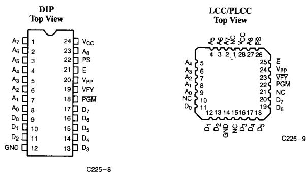
Figure 1. Programming Pinouts
