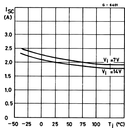
Figure 13 : Short Circuit Current vs Temperature (L4940V5)
