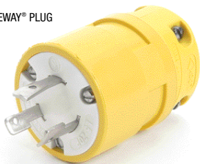
SUPER-SAFEWAY® PLUG
