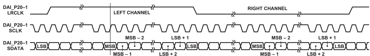
Figure 25. Right-Justified Mode
