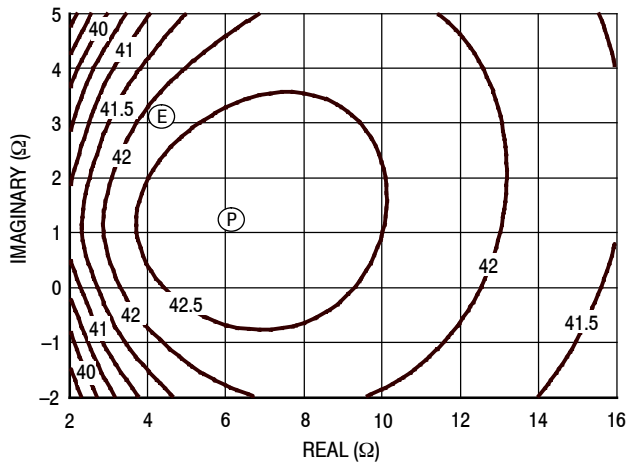
Figure 3. P3dB Load Pull Output Power Contours (dBm)
