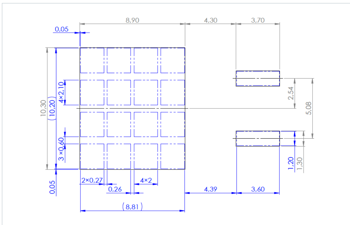
Figure 16. D 2 PAK stencil definitions(dimensions are in mm)
