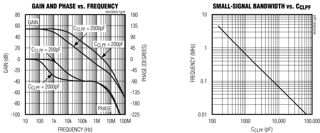
Figure 4. Gain and Phase vs. Frequency
