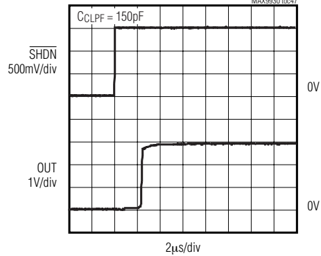
\overline{SHDN} POWER-ON DELAY RESPONSE TIME
