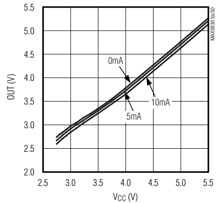
MAXIMUM OUTPUT VOLTAGE vs. V_{CC} BY LOAD CURRENT
