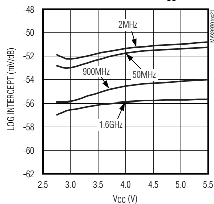
MAX9931 LOG INTERCEPT vs. V_{CC}
