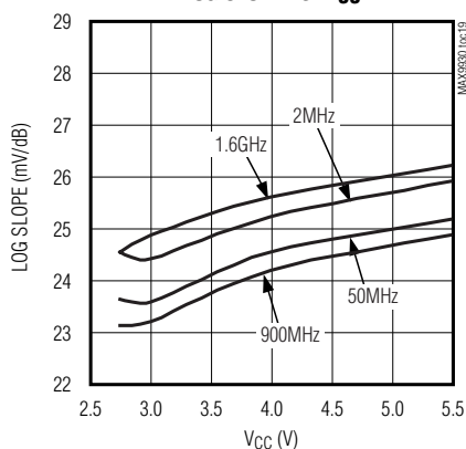
MAX9931 LOG SLOPE vs. V_{CC}
