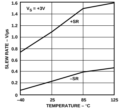
Figure 16. Slew Rate vs. Temperature, V_S = +3\text{ V}
