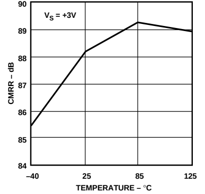
Figure 13. CMRR vs. Temperature, V_S = +3\text{ V}
