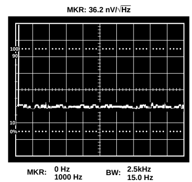
Figure 19. Voltage Noise Density, V_S = +3\text{ V} to \pm 5\text{ V} , A_{VO} = 1000
