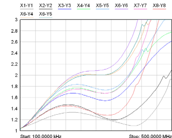
40-726A-511-L (50Ω Version) VSWR Plot to 500MHz
