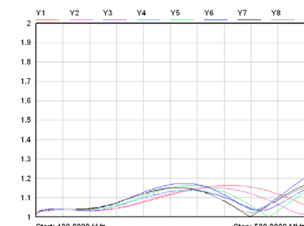
40-726A-511-L (50Ω) Loop-Thru VSWR to 500MHz
