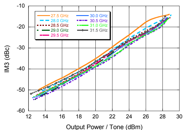
IM3 Level vs. P_{OUT} (dBm/toner)
