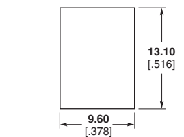
Recommended Panel Cutout Max. Panel Thk. 1.7 [0.067]
