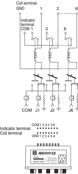
Fail-safe type
