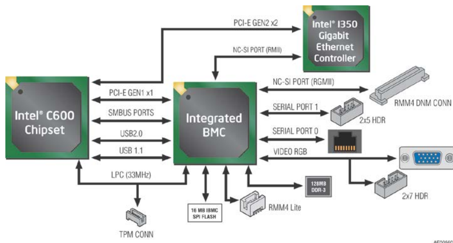
Figure 21. Integrated Baseboard Management Controller (BMC) Overview
