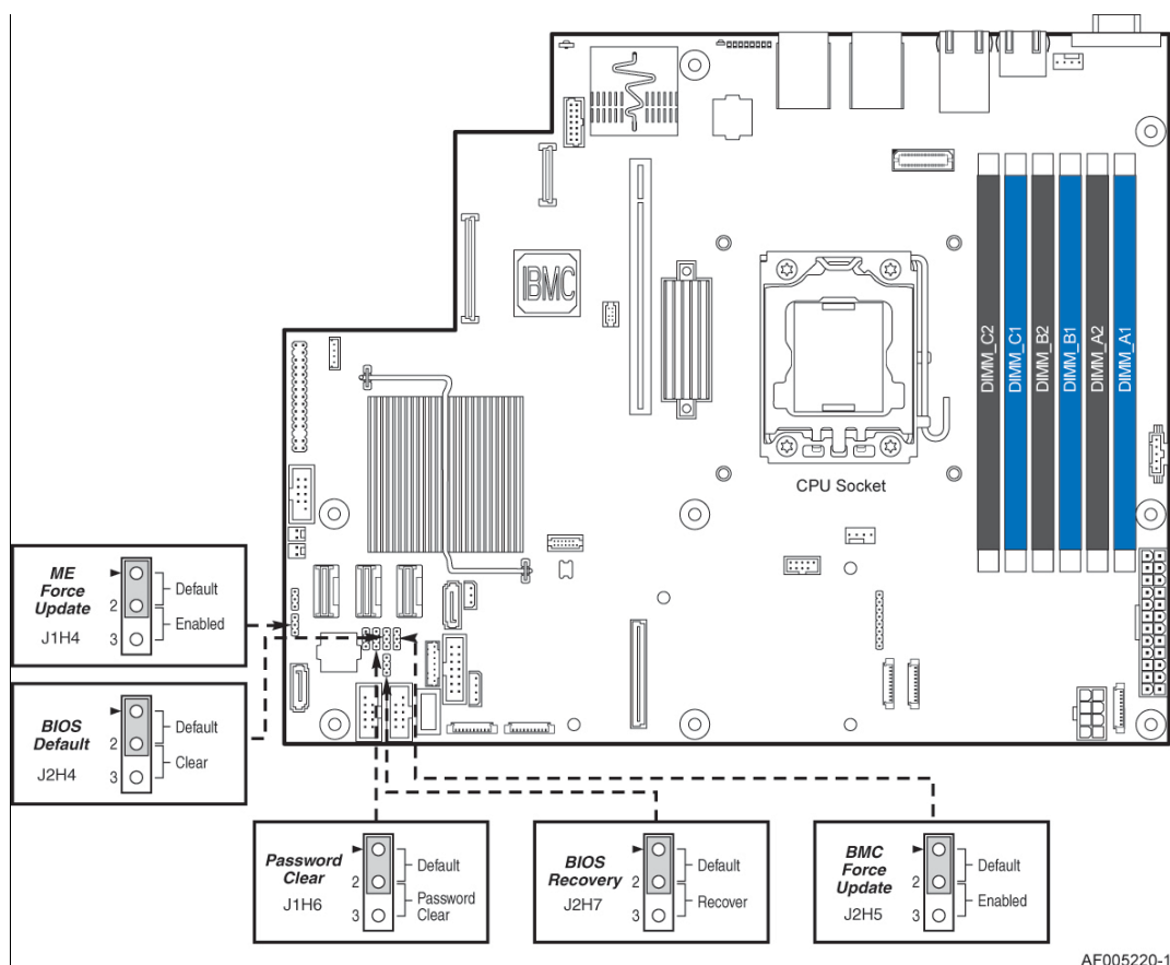
Figure 23. Jumper Blocks
