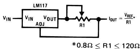
Figure 48. Precision Current Limiter
