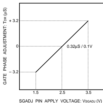
Fig. 8 Sync-gate phase
