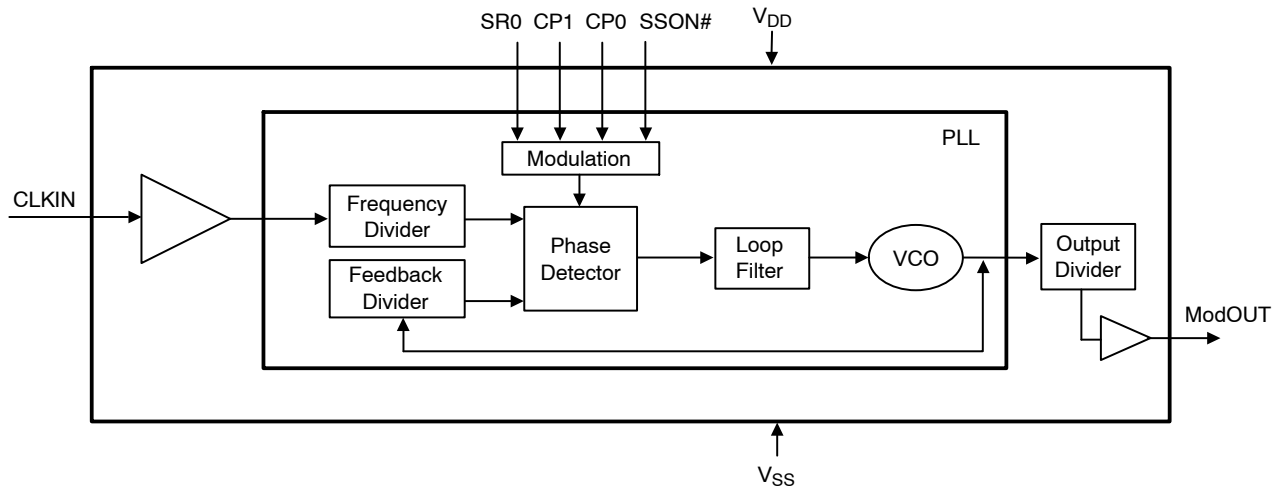
Figure 1. Block Diagram
