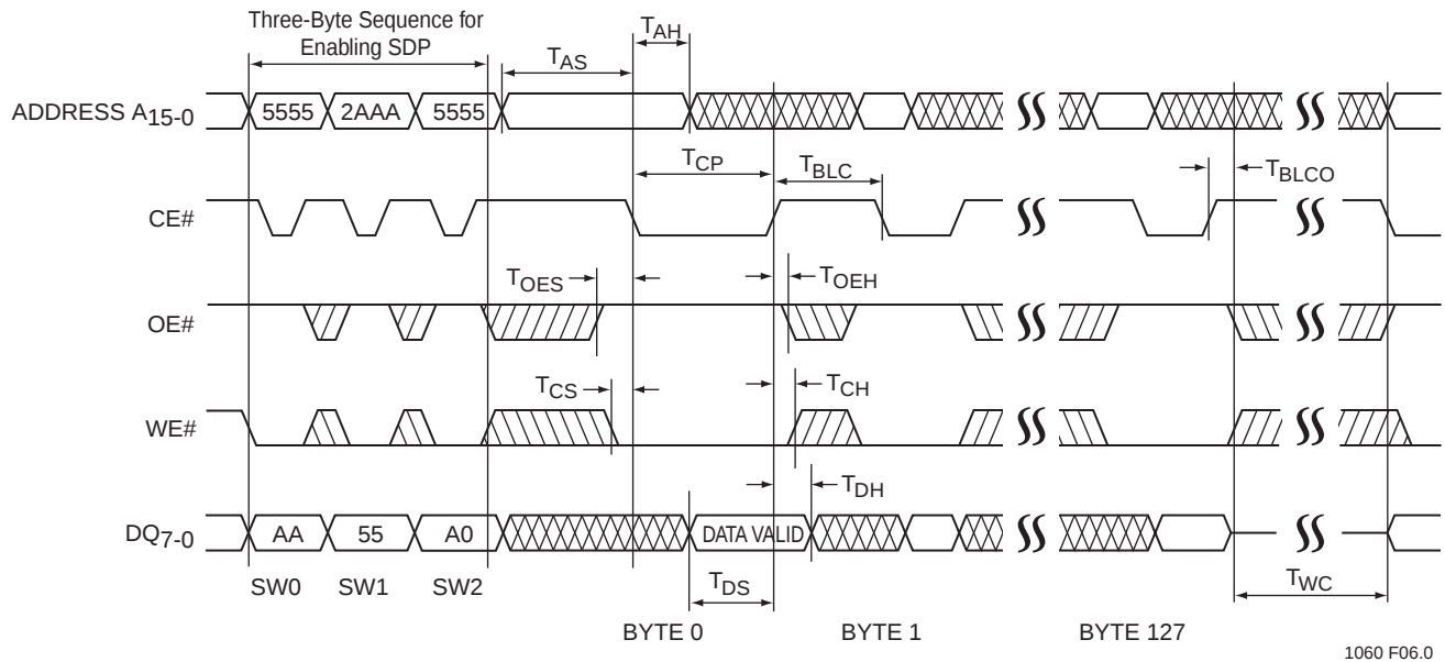
FIGURE 6: CE# CONTROLLED PAGE-WRITE CYCLE TIMING DIAGRAM
