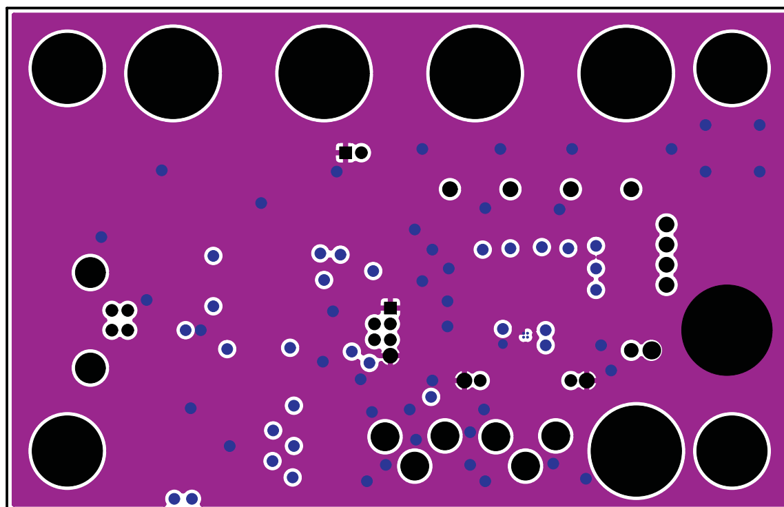
Figure 8. TPA2016D2EVM – Layer 2
