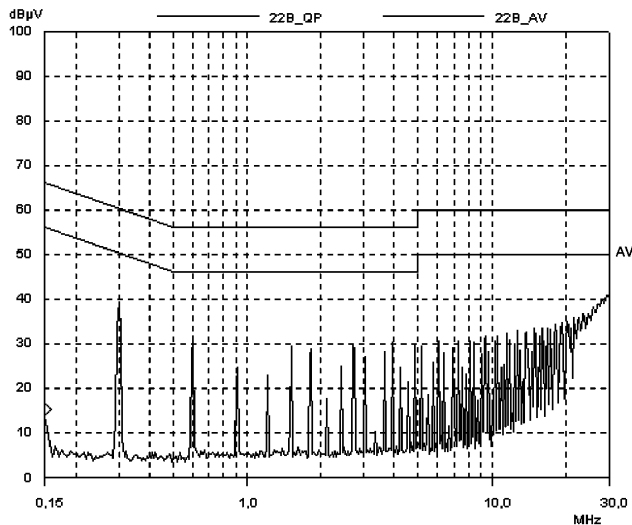
PKF 4211A with 51 \mu H common mode and 10 \mu H series inductor
