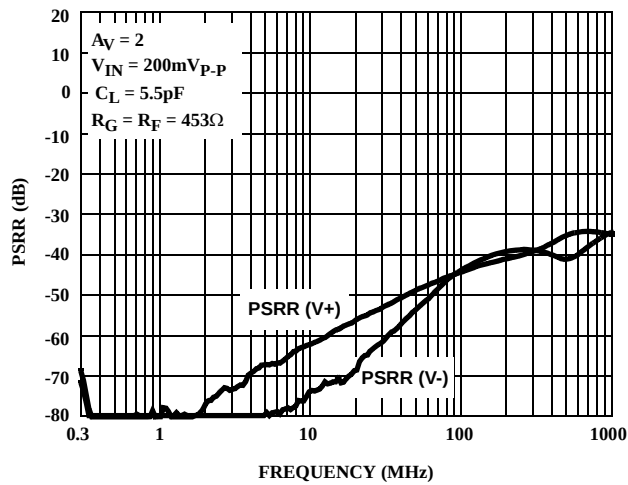
FIGURE 10. PSRR CHANNELS
