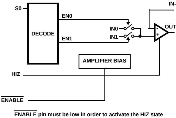
FIGURE 1. FUNCTIONAL DIAGRAM
