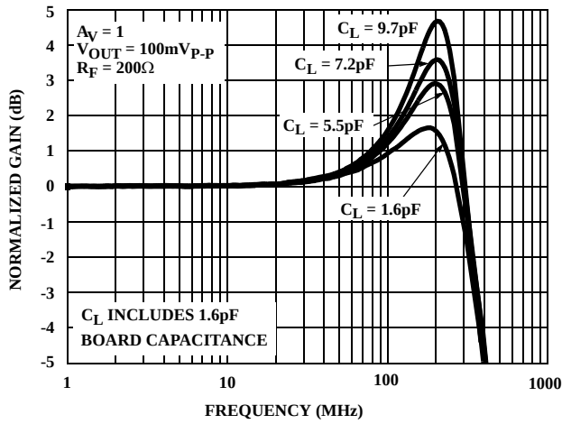
FIGURE 2. SMALL SIGNAL GAIN vs FREQUENCY vs C_L
