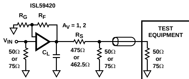
FIGURE 25A. TEST CIRCUIT FOR MEASURING WITH A 50Ω OR 75Ω INPUT TERMINATED EQUIPMENT
