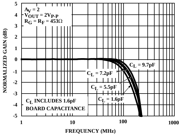
FIGURE 4. LARGE SIGNAL GAIN vs FREQUENCY vs C_L
