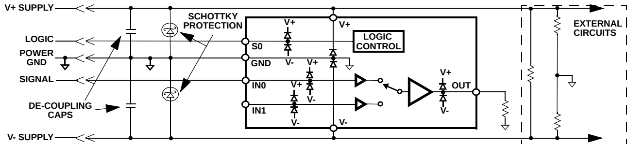
FIGURE 27. SCHOTTKY PROTECTION CIRCUIT
