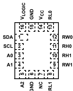
ISL23328 (16 LD UTQFN) TOP VIEW
