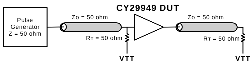
Figure 1. LVMOS_CLK CY29949 Test Reference for V_{CC} = 3.3V and V_{CC} = 2.5V
