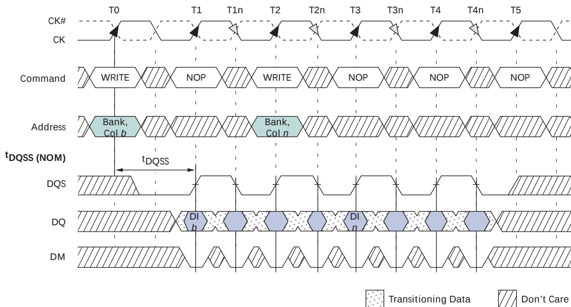
Figure 39: Consecutive WRITE-to-WRITE
